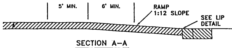
TYPICAL CURB RAMP
